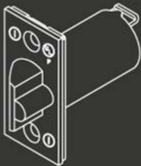
Deadlatch 1/2" Throw 2 1/4" × 1"
